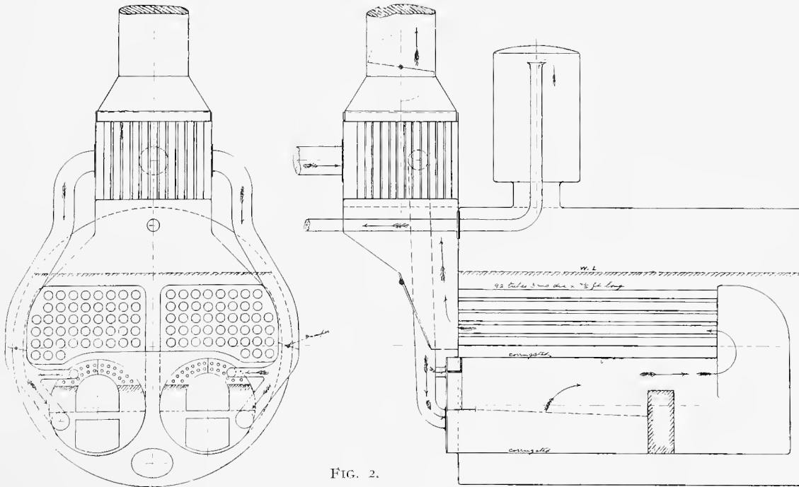
ENGINES AND BOILER OF STEAM YACHT NEAIRA.
